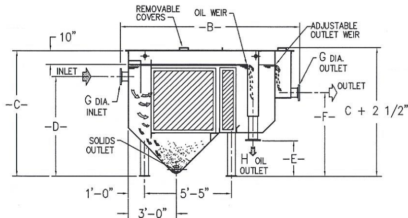
SECTIONAL ELEVATION VIEW
