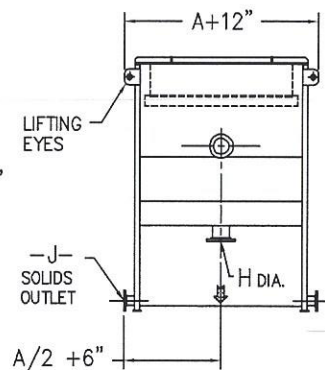
END VIEW
